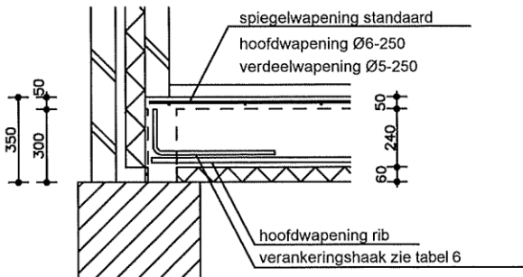
detail ribwapening
