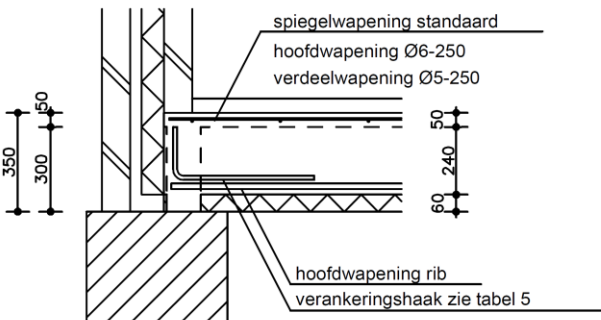
detail ribwapening
