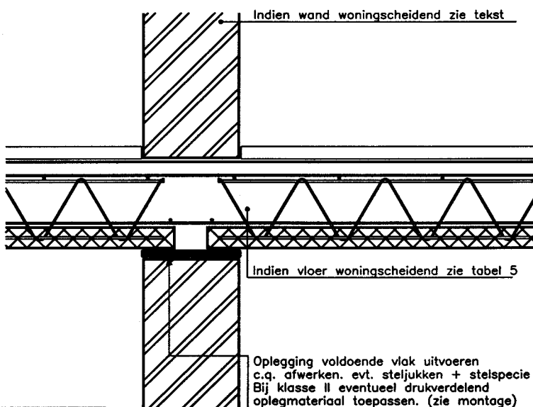
Detail IIa
