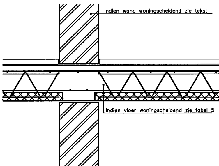
Detail II
