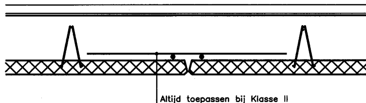
Detail VIII
